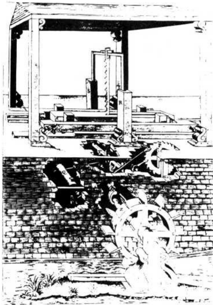
Figure 16. Water-driven sawmill as depicted by Ramelli in 1588.
