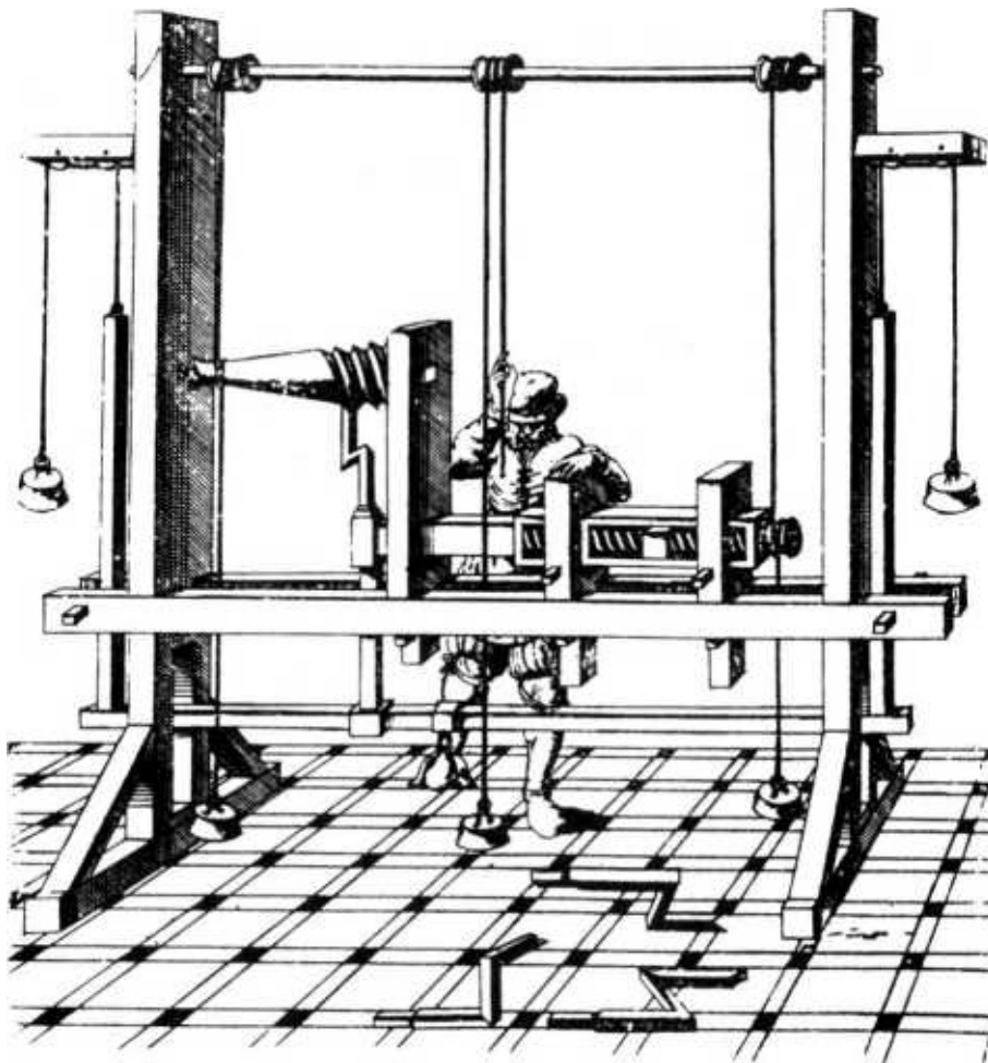
Figure 20. Jacques Besson's screw-cutting lathe, dating from 1579.
