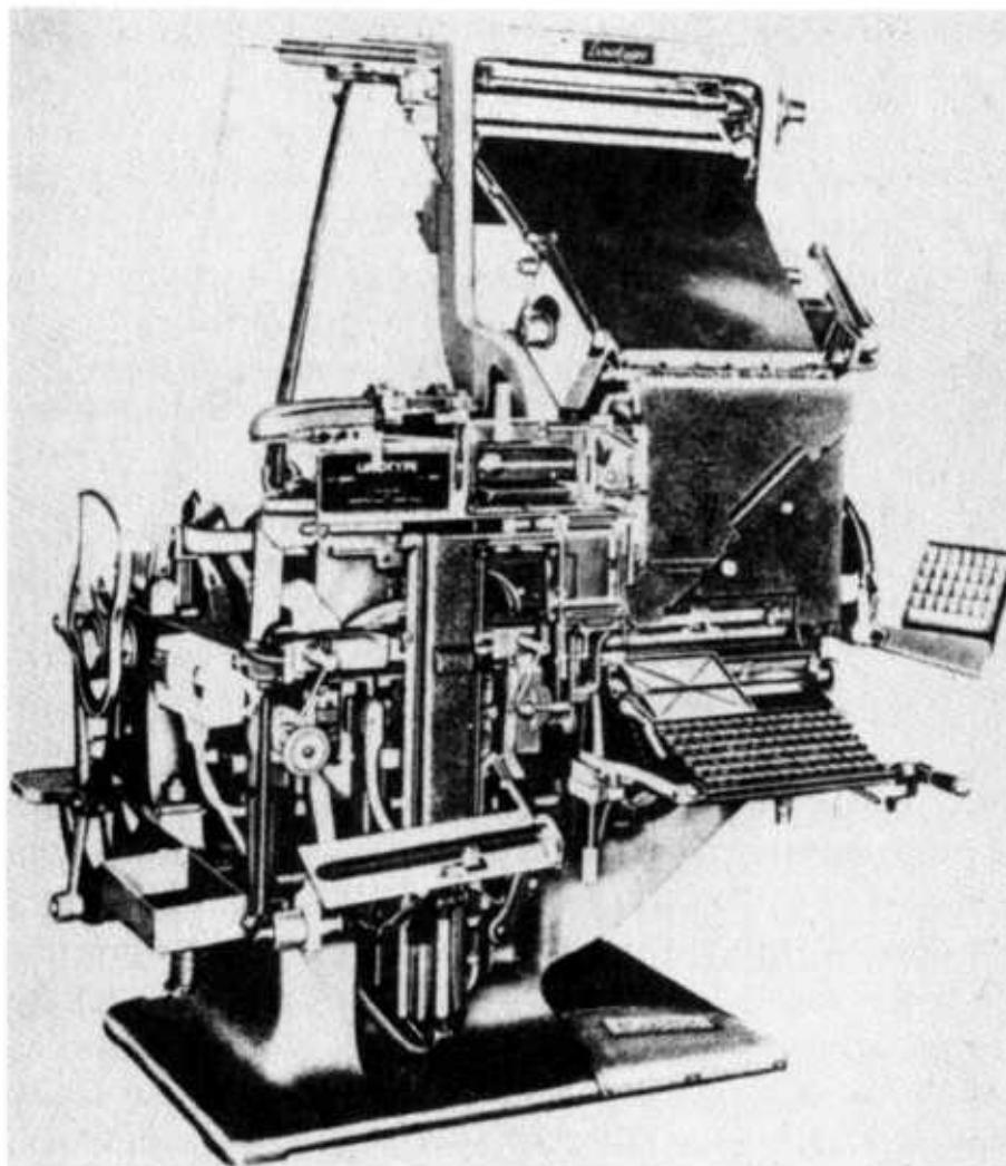
Figure 39. Linotype machine, invented by Mergenthaler. The keyboard controlled bronze letters that were set on a line, used as a mold on which molten type-metal was poured and then used as type.
