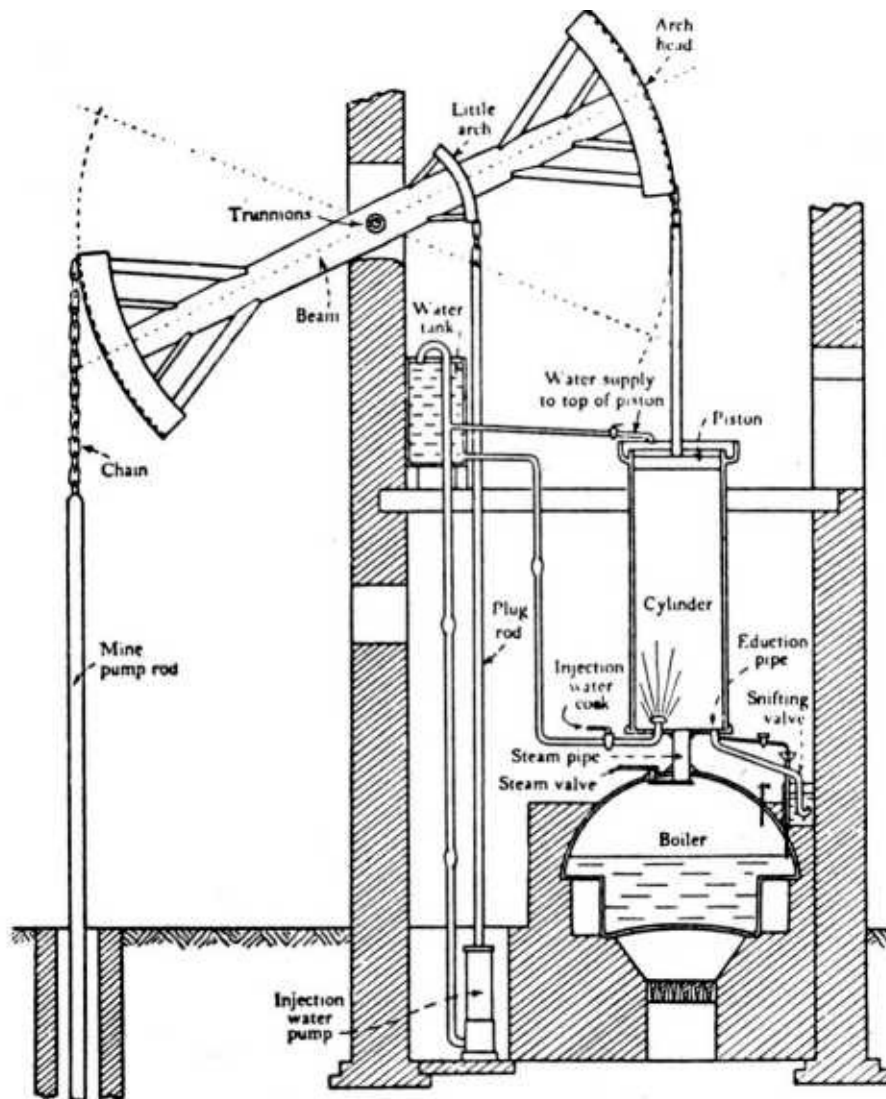
Figure 23. Diagram of Newcomen's atmospheric engine.
