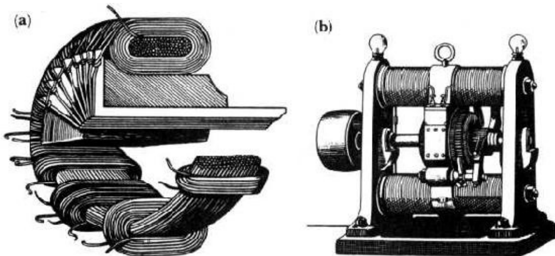
Figure 34. The first successful dynamos, built by Z.T. Gramme. On the left, typical ring armature, on the right, commercially made dynamo (1874). Source: (a) After J. Dredge (ed.). 'Electric Illumination,' Vol. I, Fig. 125. London, Offices of Engineering, 1882. I). E. Woodall. (b) After S. P. Thompson. 'DynamoElectric Machinery' (3rd ed., enl. and rev.), Fig. 87. London, Spon, 1888. 1). E. Woodall.
