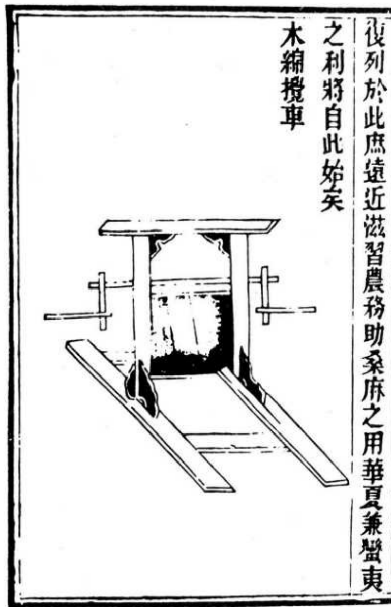
Figure 43. Chinese cotton gin, in use during the Yuan dynasty (thirteenth to fourteenth centuries). Source: Nung Su, 1313.
