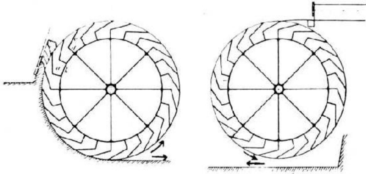
Figure 25. Comparison of high breast waterwheel (left) and traditional Waterwheel (on the right). Note that in the breast-wheel the water moves in the same direction as the wheel, in contrast with the traditional wheel.
