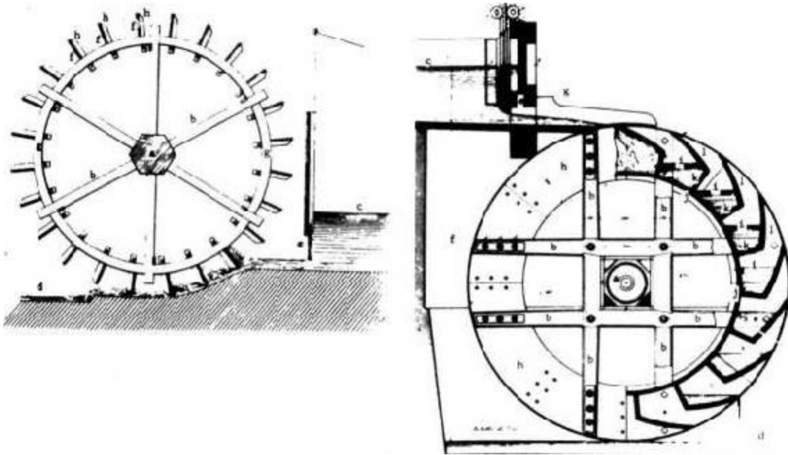
Figure 5. Main types of the waterwheel: undershot wheel (left) and overshot wheel (right).
