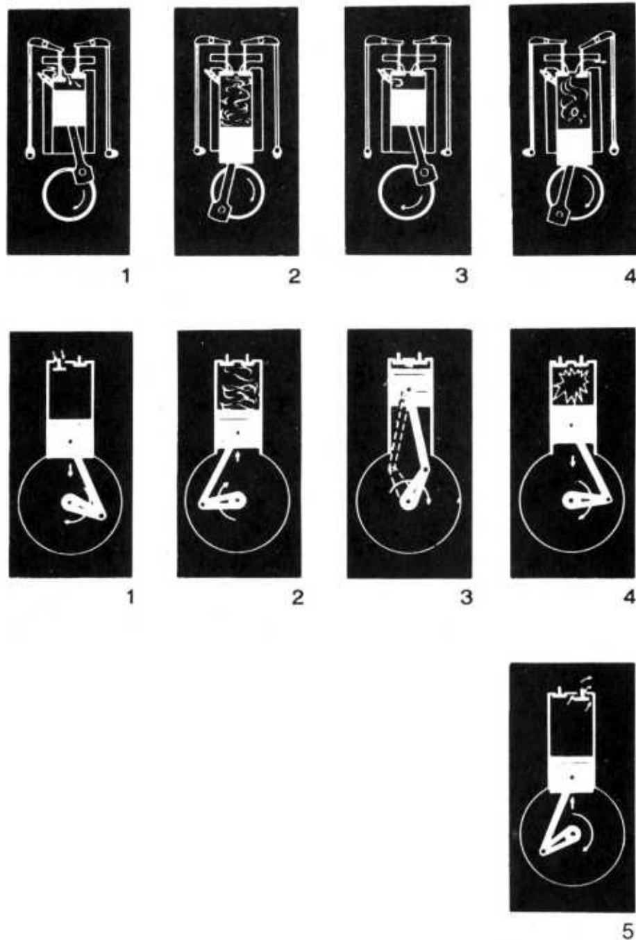
Figure 37. the two main types of internal combustion engines. On the top, the four stroke cycle invented by Otto. The bottom shows the five stages of the compression-ignited Diesel engine.
