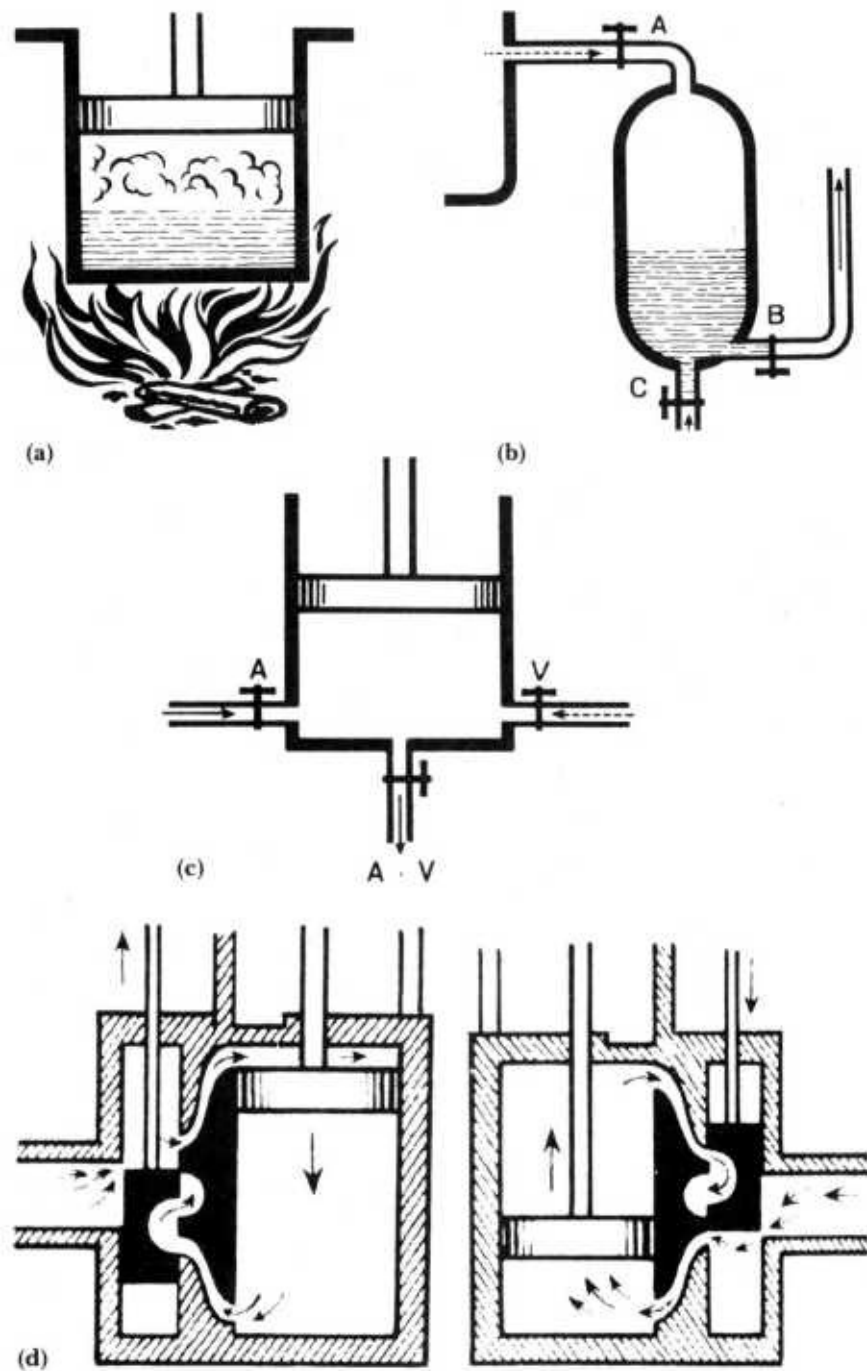
Figure 24. Principles of early steam engines: (a) Papin's prototype, (b) Savery's pistonless suction pump, (c) Newcomen's engine, and (d) Watt's double-acting engine. The machine exploits the contrary motion of the piston and the slide-valve above it, with the steam entering alternately from the left and the right.
