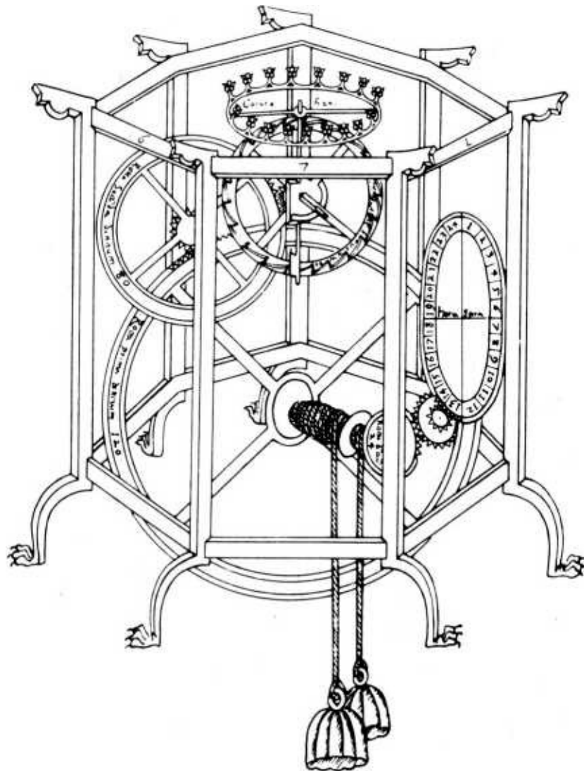
Figure 12. Astronomical clock designed by Giovanni Dondi in 1364.
