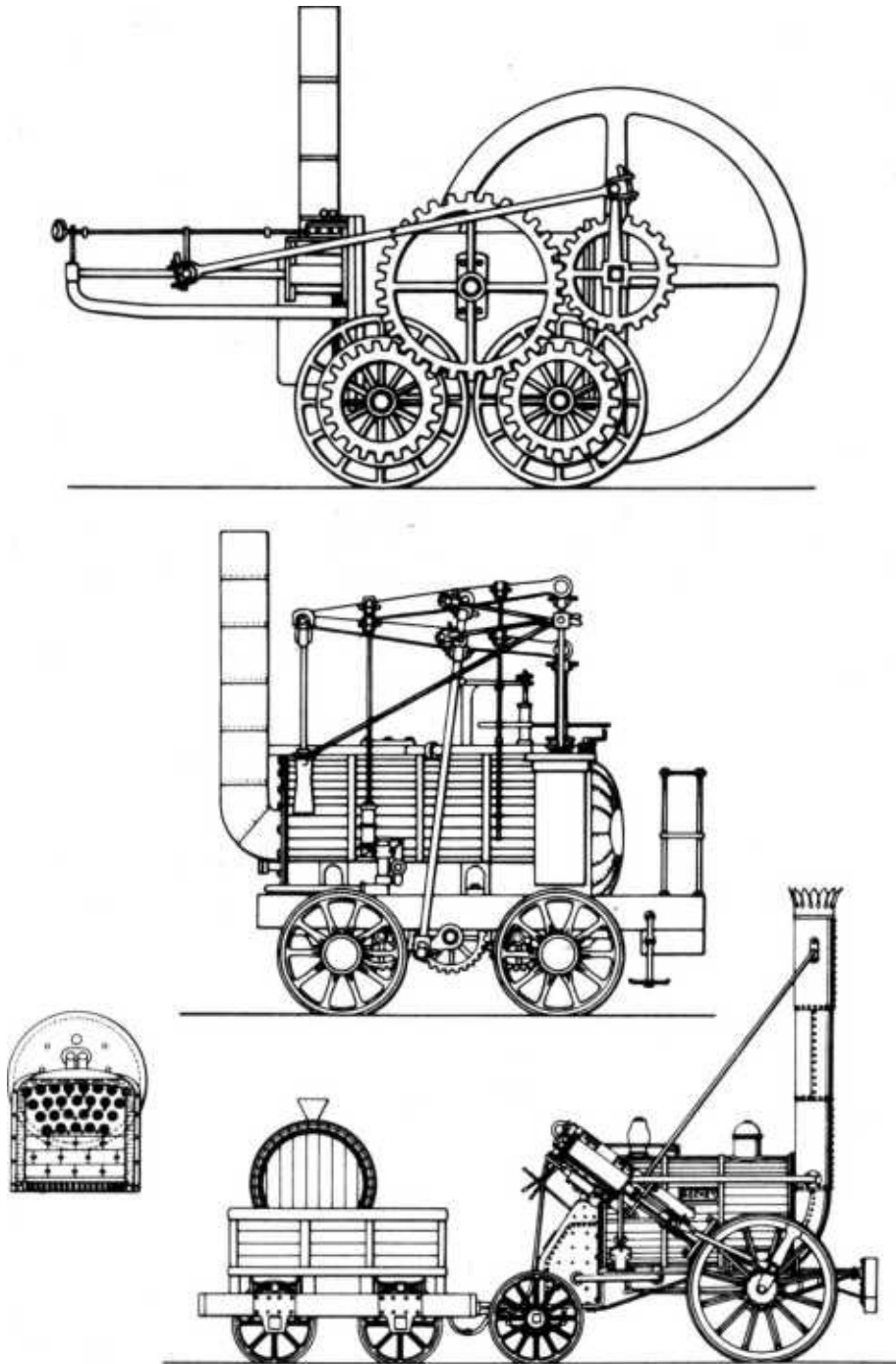
Figure 35. Early high-pressure engines: first Trevithick locomotive, 1803; William Hedley's "puffing Billy," used in collieries; Stephenson's Rocket, which won the Rainhill competition.
