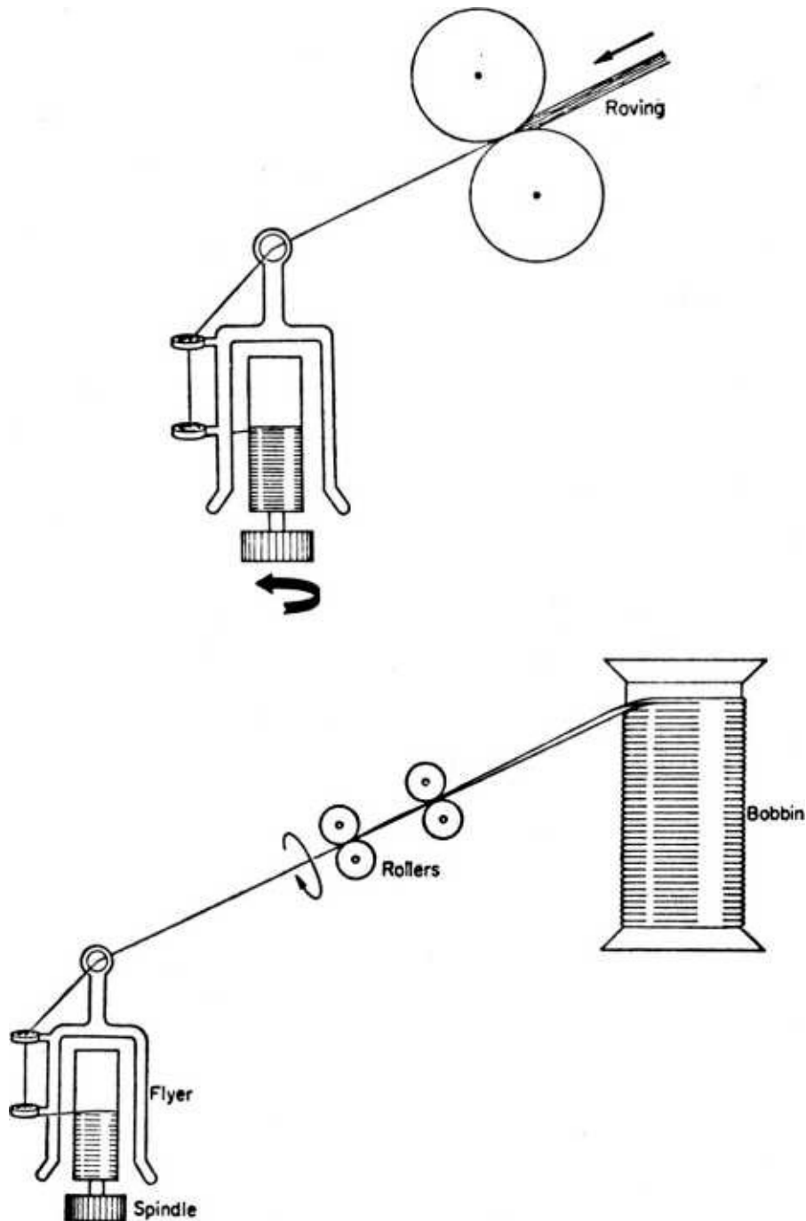
Figure 27. The mechanical principle behind the Wyatt-Paul spinning machine,
