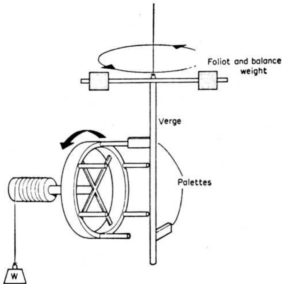
Figure 11. Principle of the weight-driven clock. The weights on top of the foliot ensure that the power of gravity is uniform. The palettes help convert the uniform pull of the weight into the oscillating motion needed for the clock.
