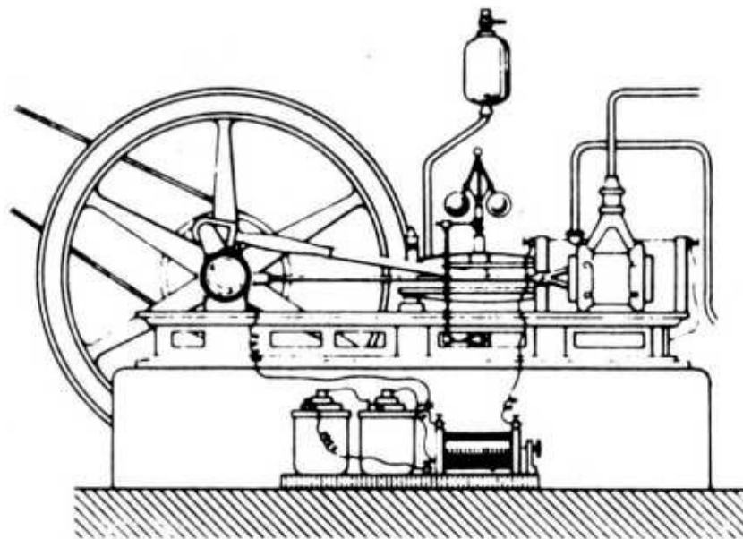
Figure 36. Gas engine, built by Lenoir in 1860.
