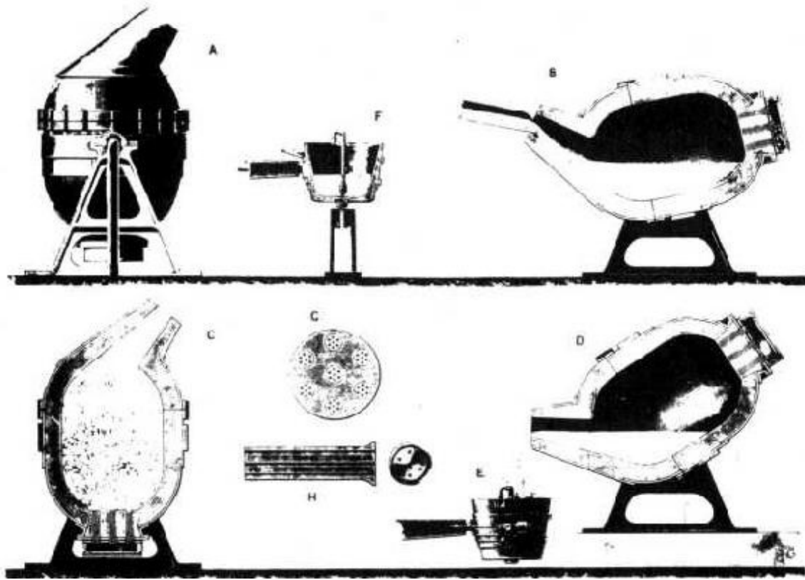
Figure 33. Drawing of an early Bessemer converter (1860). The airblast is introduced through the holes in the bottom. After the blast at (C), the steel is poured into the ladle (E).
