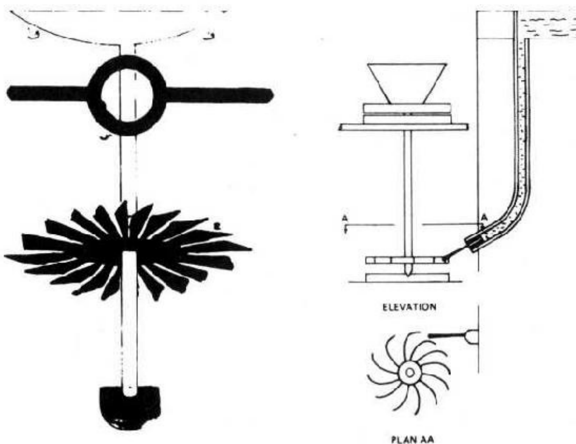
Figure 9. Horizontal waterwheel as described by the Islamic writer al-Jazari. The left shows a thirteenth-century illustration; the right shows a modern reconstruction.
