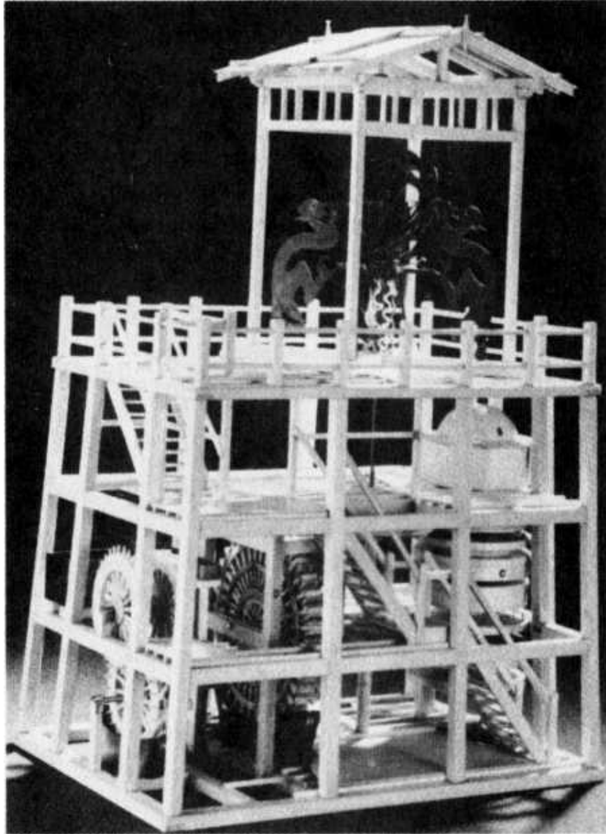
Figure 46. Model of the "Great Cosmic Engine" made by Su Sung ill 1086. The clock had it mechanical escapement, but was turned by water power.
