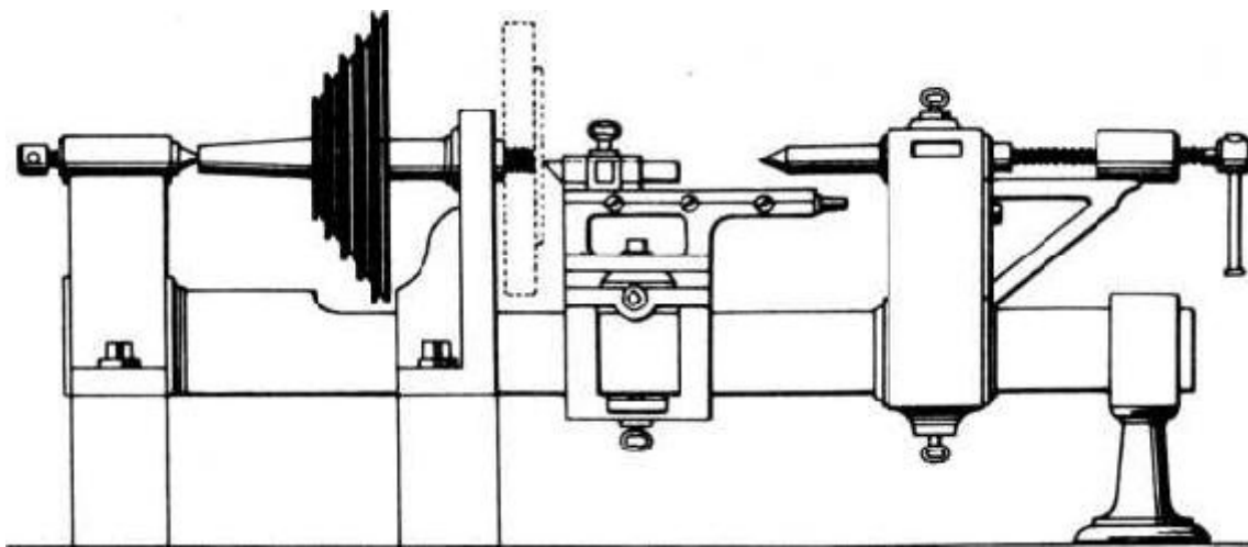
Figure 31. Henry Maudslay's slide and finishing lathe, dating from 1800. Source: Maurice Dauras, A History of Technology and Invention , Vol. III, Crown Publishers Inc., New York.
